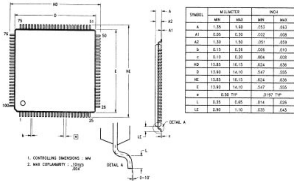
100-Lead VQFP Package Diagram
